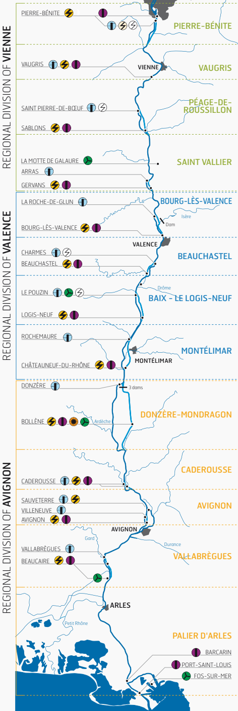
A typical CNR development scheme: 18 out of CNR's 19 hydropower plants have low heads. The low storage capacities of the reservoirs are used to modulate flow rates and thus optimise production.
